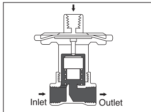
Figure 11A: Normally Open, Operator Exhausted
