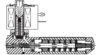
5/2 function, monostable
